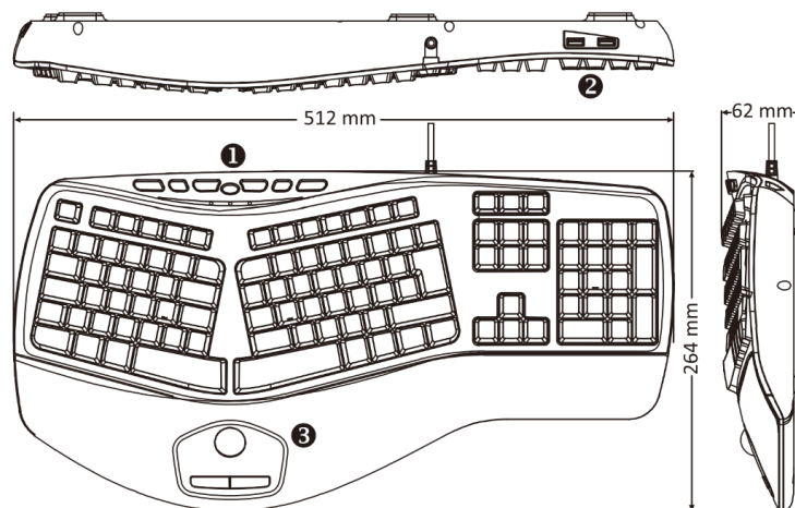
① Hotkeys ② 2xUSB Hub ③ 25mm Trackball with Left/Right Click
